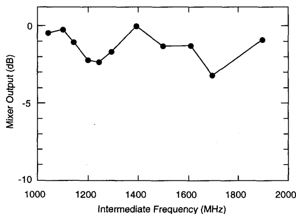
Fig. 6. The heterodyne output power of the bolometer as a function of intermediate frequency.
